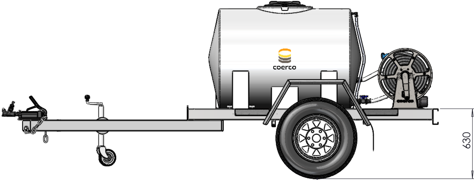
SIDE VIEW
