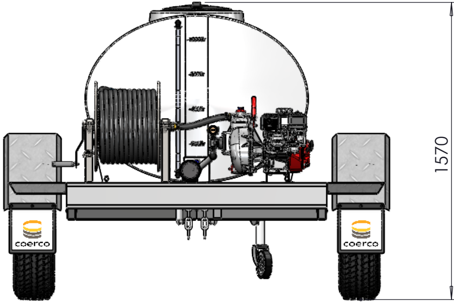
REAR VIEW
