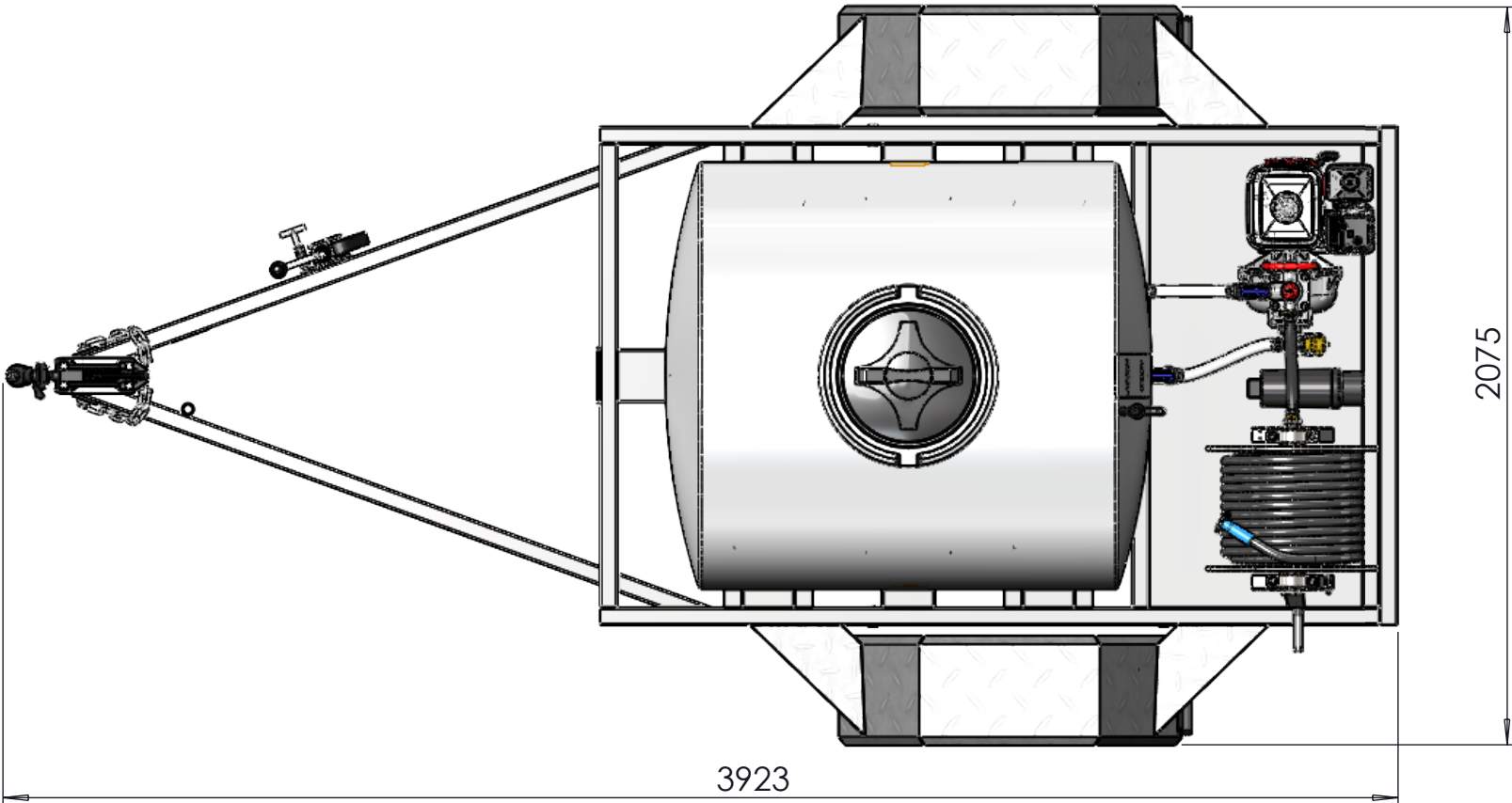
TOP VIEW
