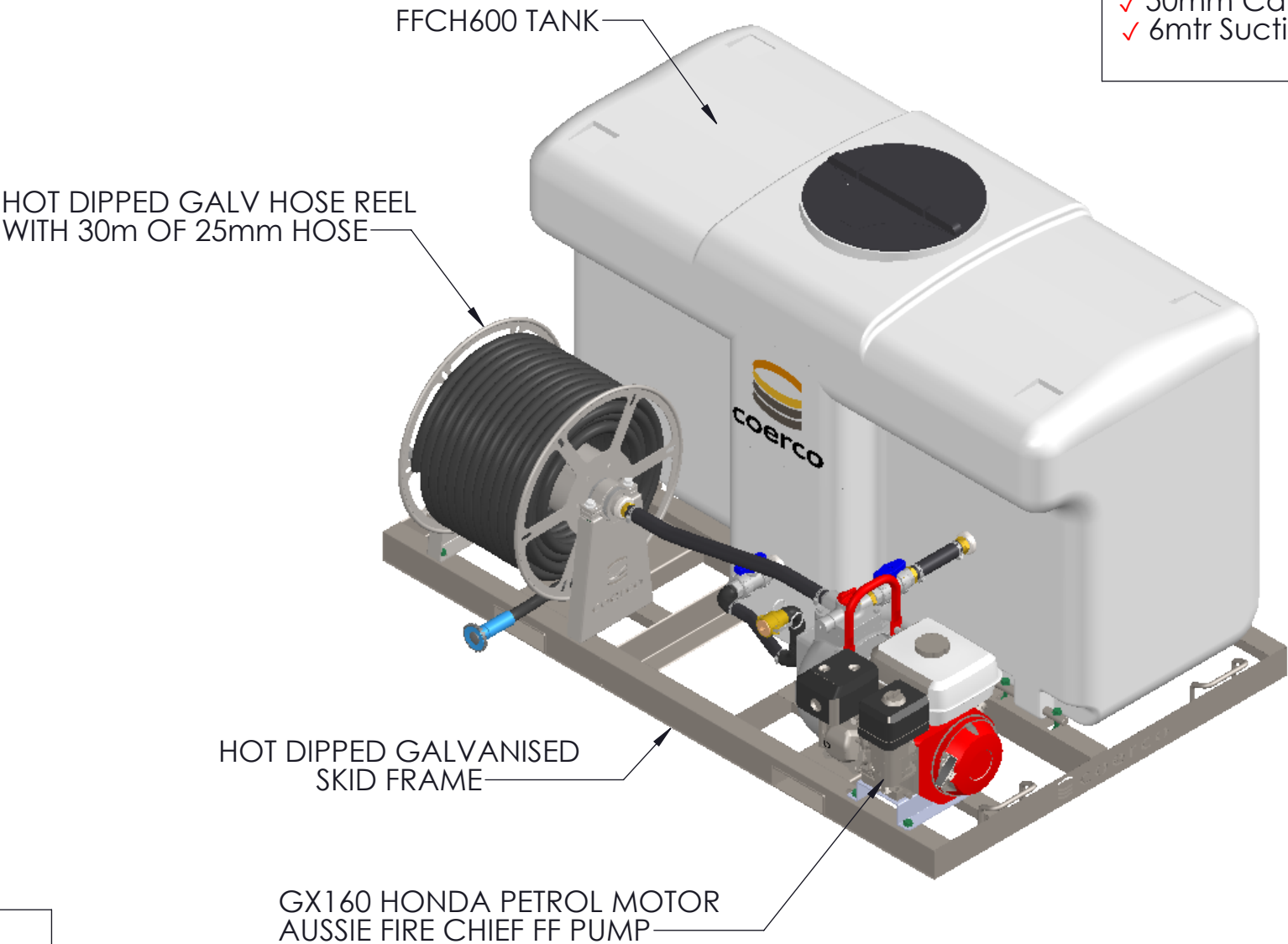
ISOMETRIC VIEW
